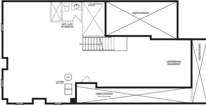
Lower Level Elev A
