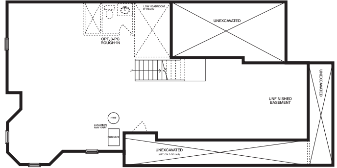
Lower Level Elev B
